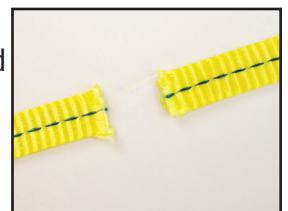
Failure due to sharp edge conditions
